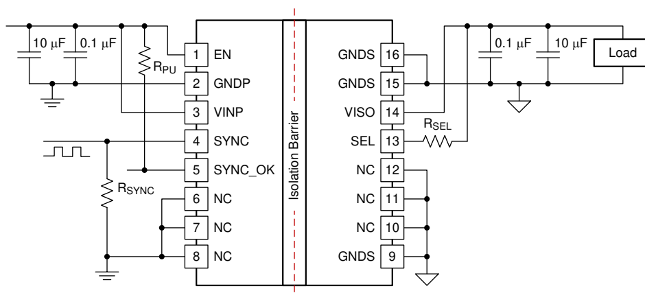
Figure 28. Typical Application
