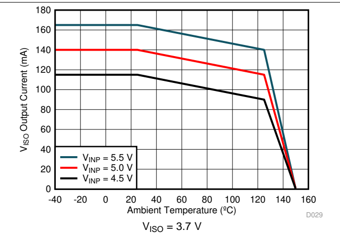
Figure 11. Maximum V ISO Output Current vs. Temperature
